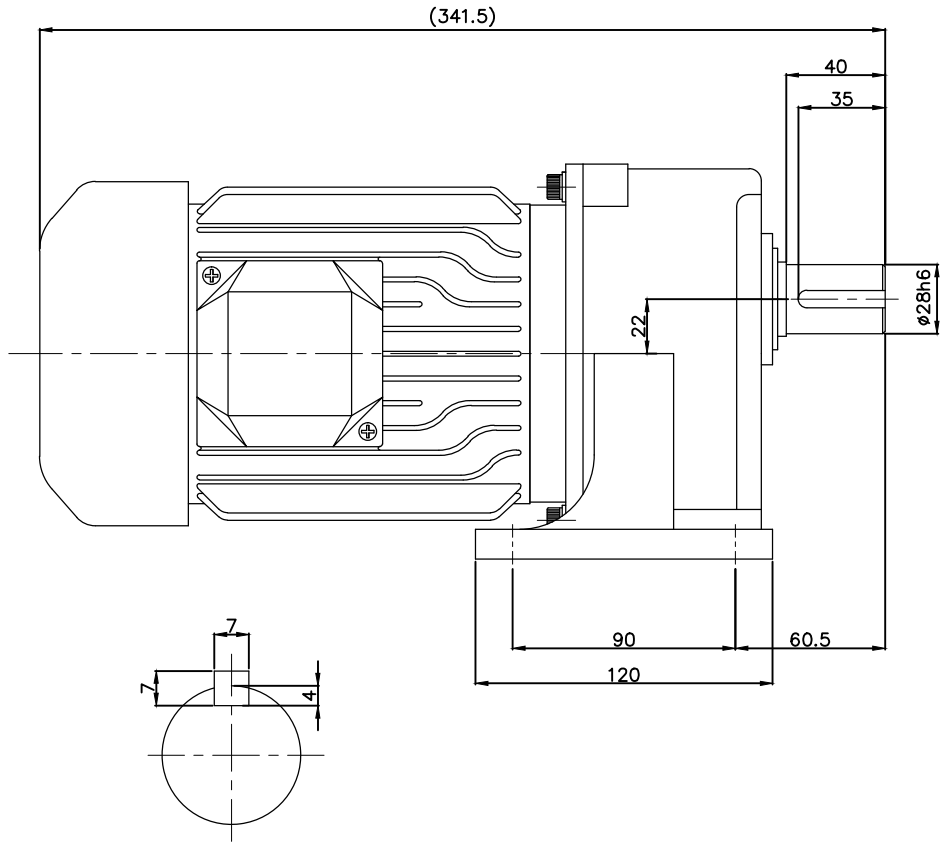
OUTPUT SHAFT
