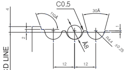
DETAIL OF GROOVE GROOVE HARDNESS HB190~220
