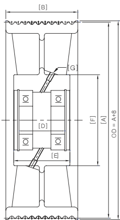
DETAIL OF GROOVE GROOVE HARDNESS HB190~220
