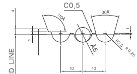
DETAIL OF GROOVE GROOVE HARDNESS HB190~220
